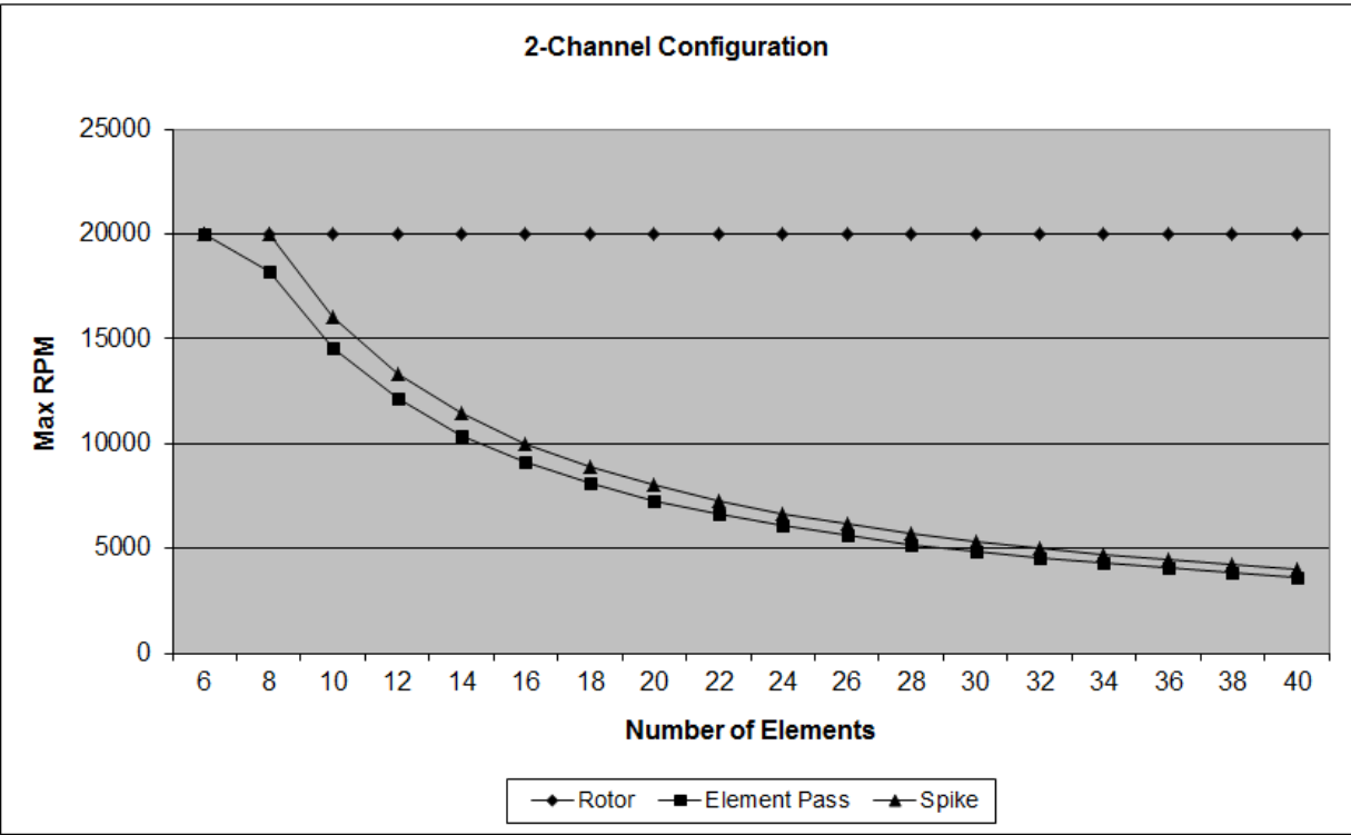
Figure 5: Only one channel of a channel pair is enabled.
